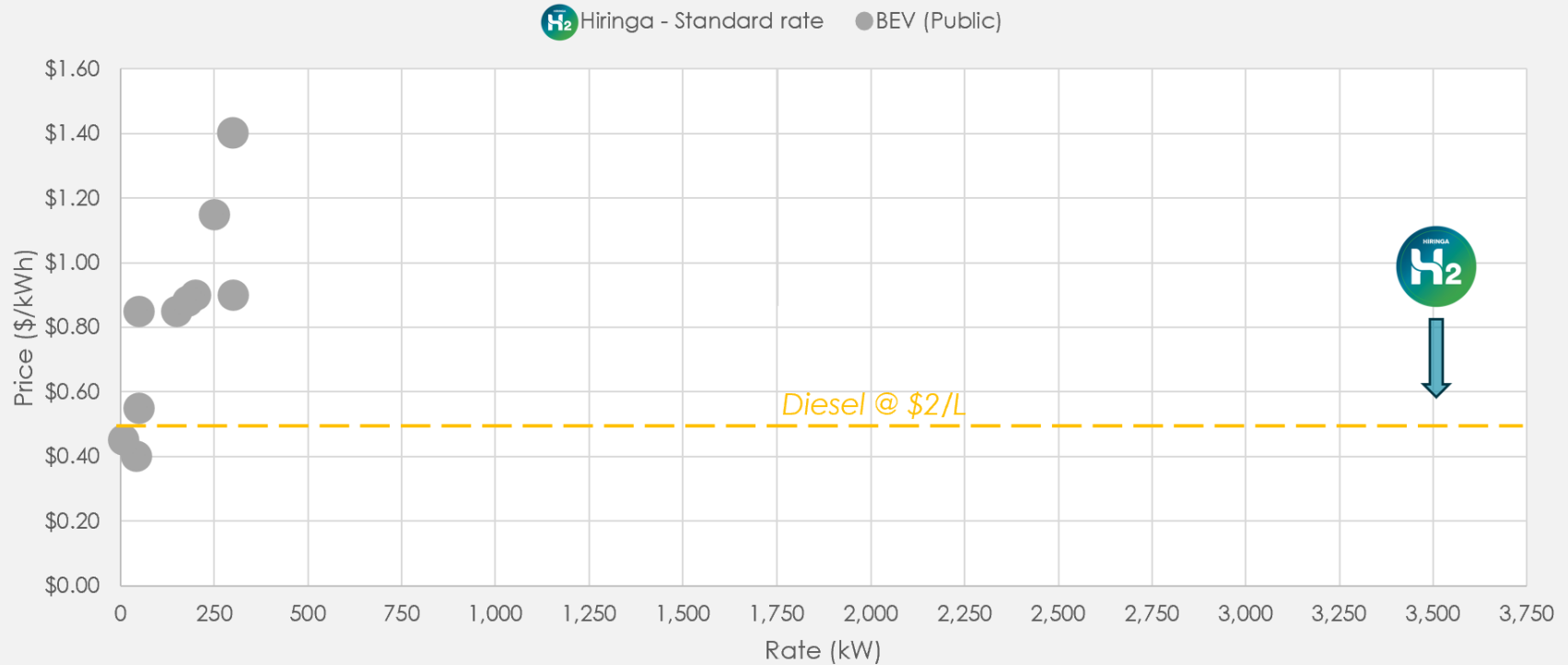
Energy Price vs Fuelling Rate for BEV and FCEV
